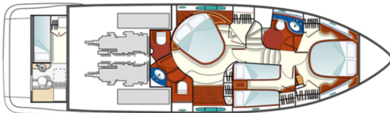
LOWER DECK
